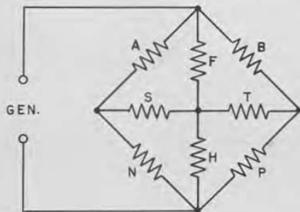
FIGURE 6. Diagram of a bridge with both guard and coupling circuits.
