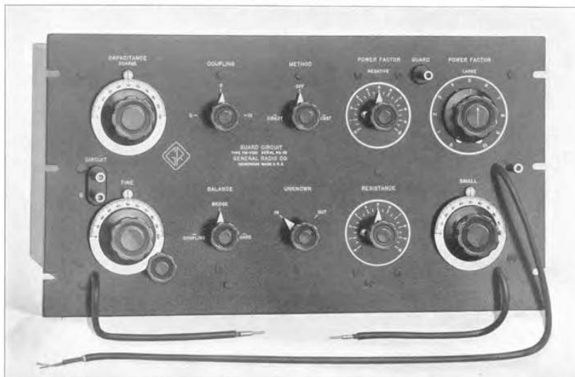
FIGURE 1. Panel view of the TYPE 716-P2 Guard Circuit.
