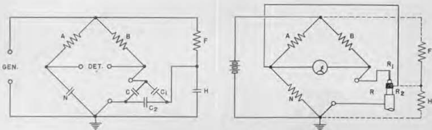
FIGURE 2. Schematic diagram showing how a guard circuit is connected to a bridge for measuring a three-terminal capacitance.
