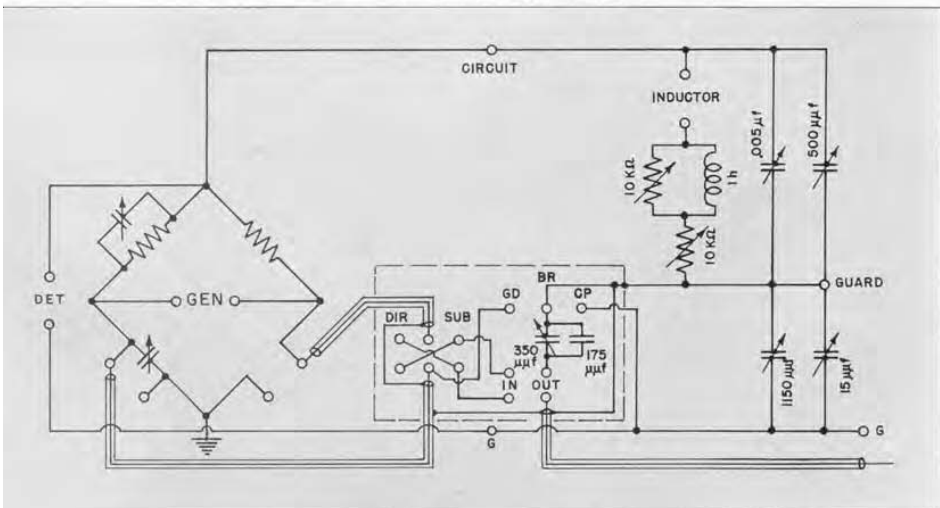
FIGURE 7. Wiring diagram of the TYPE 716-P2 Guard Circuit.
